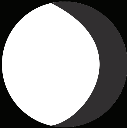
Waning Gibbous
