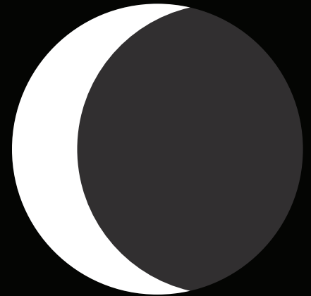
Waning Crescent
