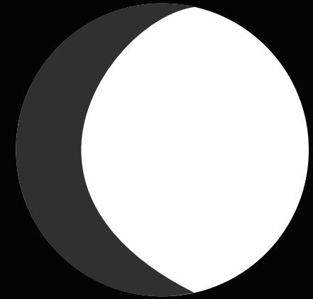
Waxing Gibbous
