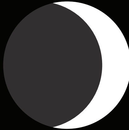
Waxing Crescent
