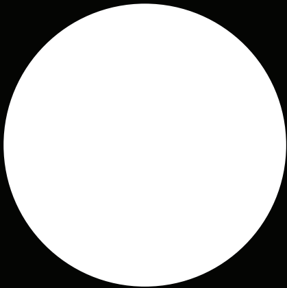
Full Moon
